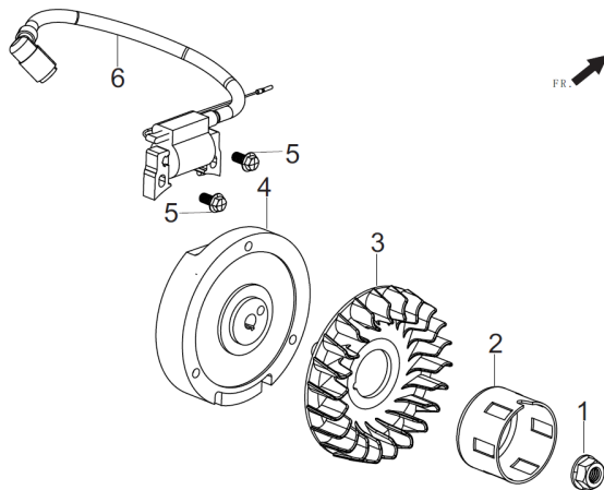
FIG.13 FLYWHEEL / IMPELLER / STARTER PULLEY / IGNITION COIL (E15)
