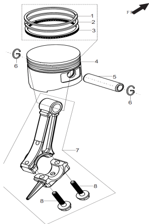
FIG.5 RING SET,OIL / ROD,CRANKSHAFT CONNETING (03)
