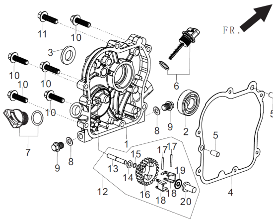
FIG.3 COVER SUBASSEMBLY, CRANKCASE (E01)
