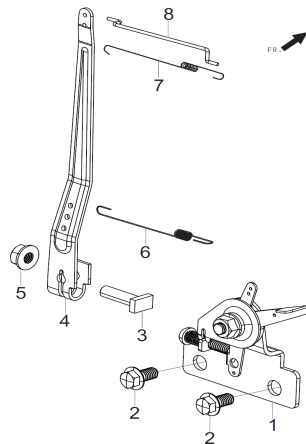
FIG.14 CONTROL ASSY, THROTTLE (E13)
