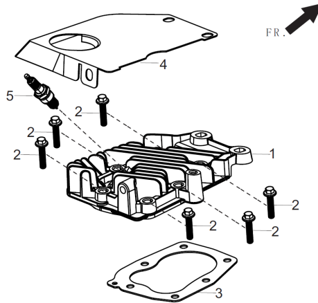
FIG.1 CYLINDER HEAD / PLUG,SPARK (E04)
