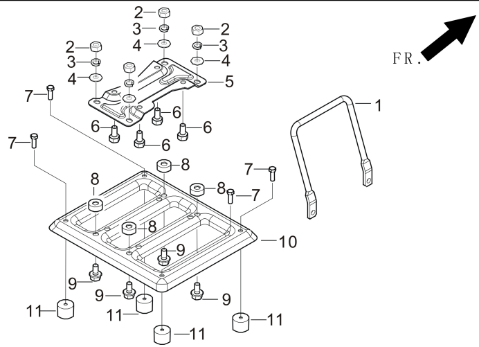
FIG.16 FRAME ASSY, ENGINE (E16)
