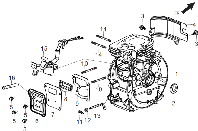
FIG.2 CRANKCASE ASSY (E17)
